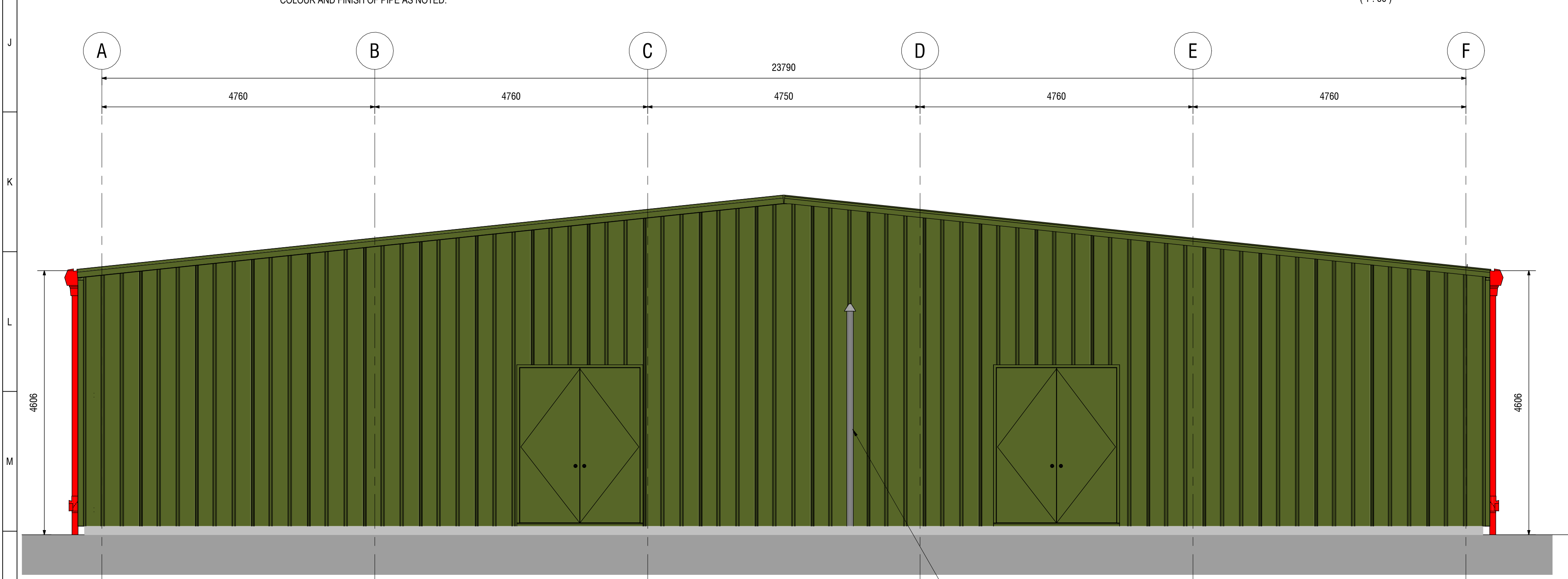
ELEVATION ON GRIDLINE 1 (1:50)
