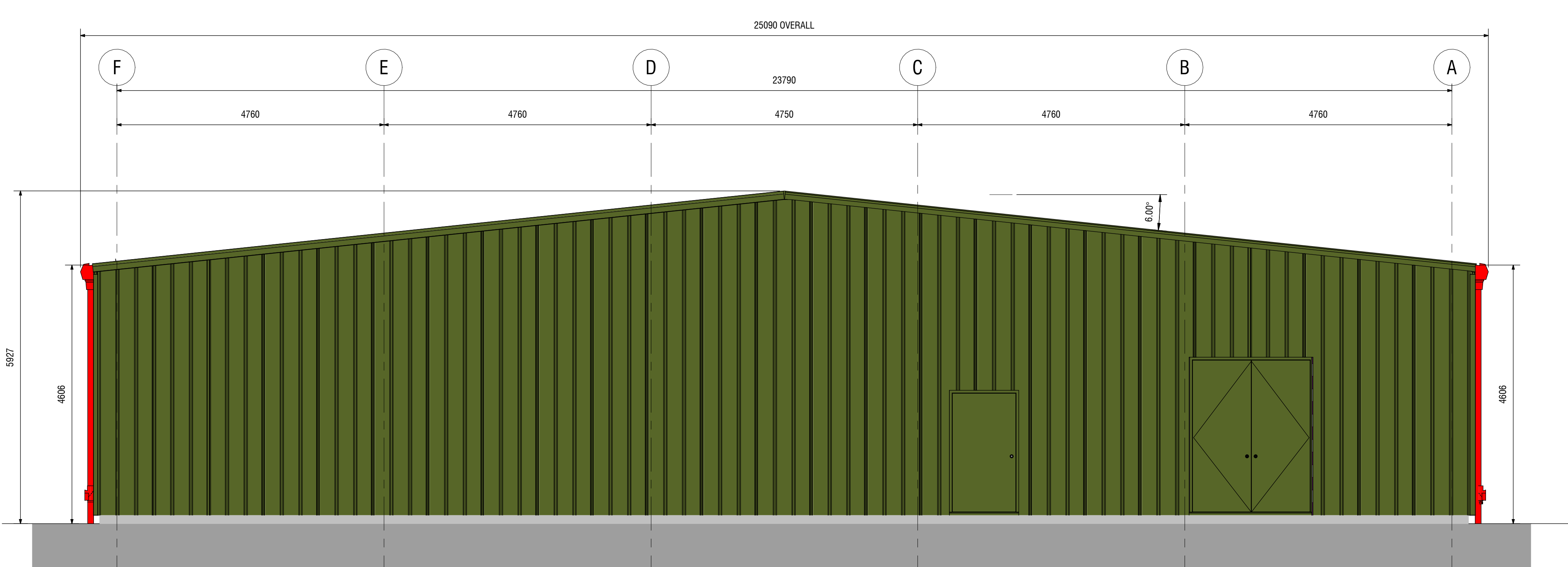
ELEVATION ON GRIDLINE 9 (1:50)
