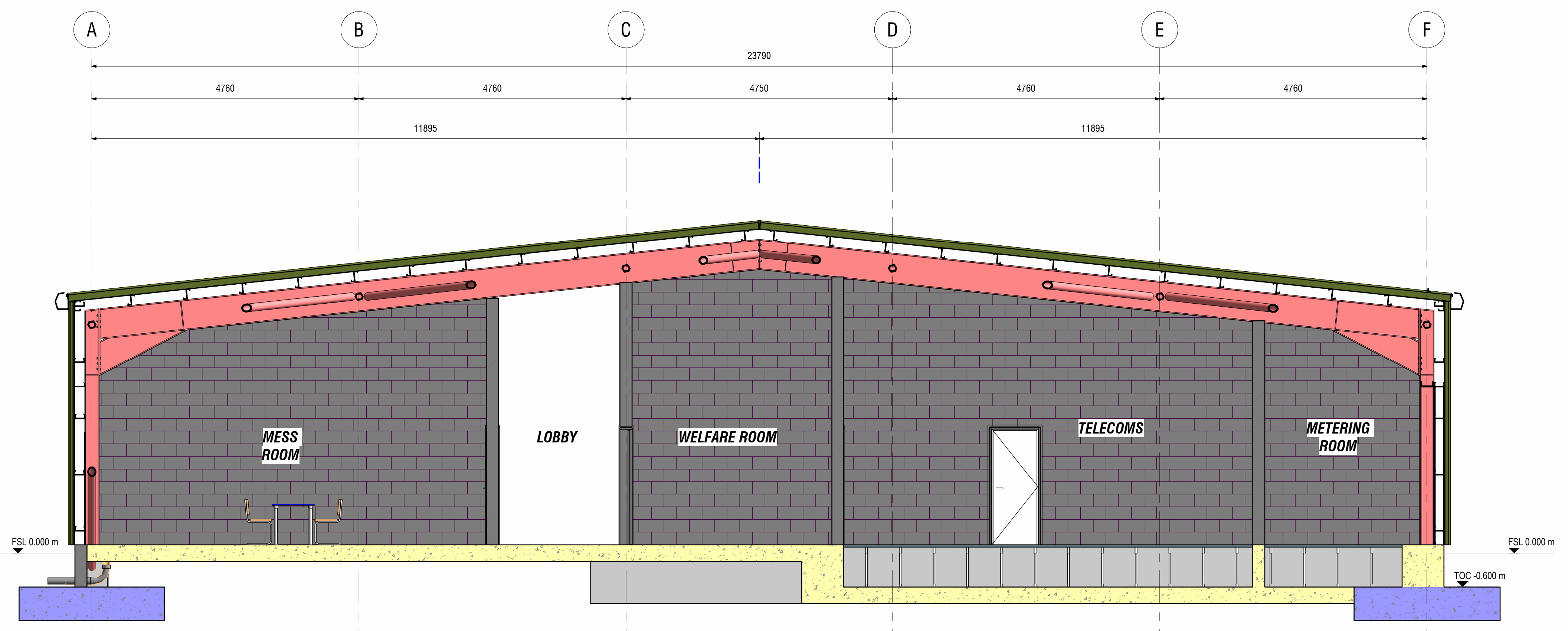
SECTION A - A (1:50)
