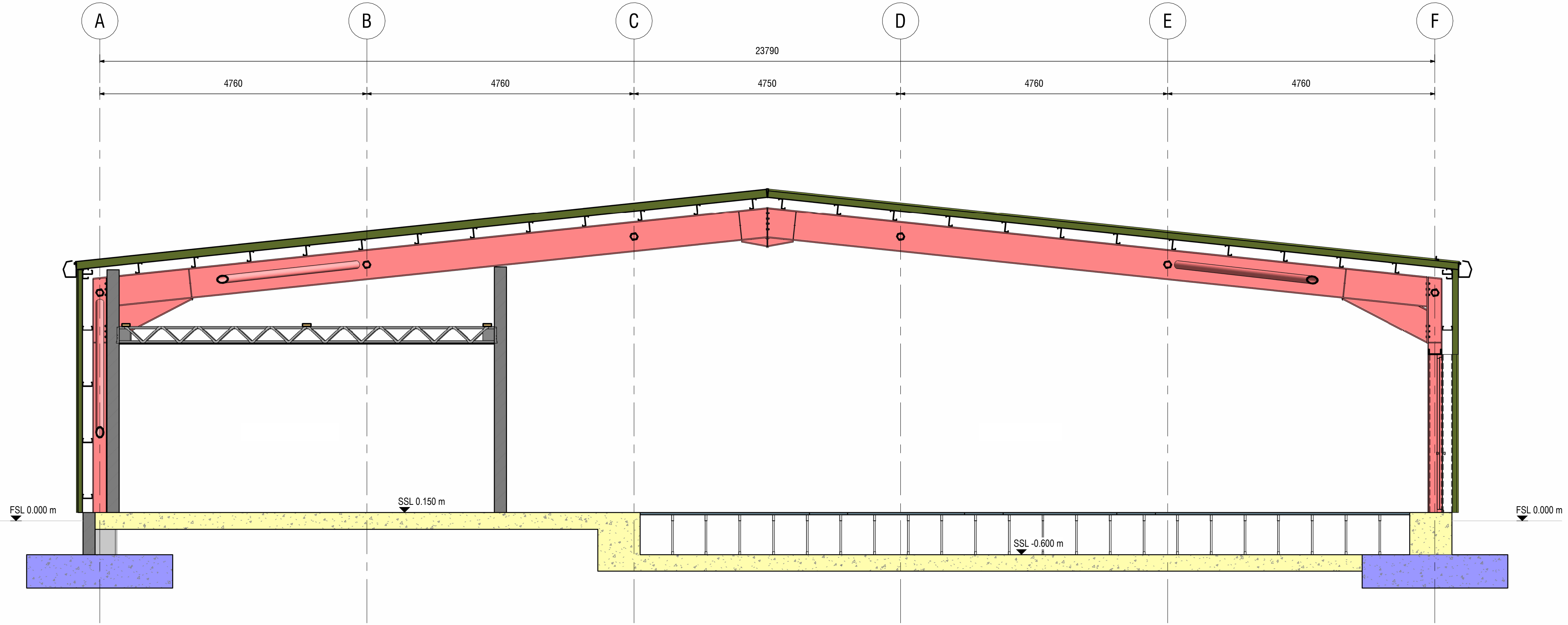
SECTION C - C (1:50)
