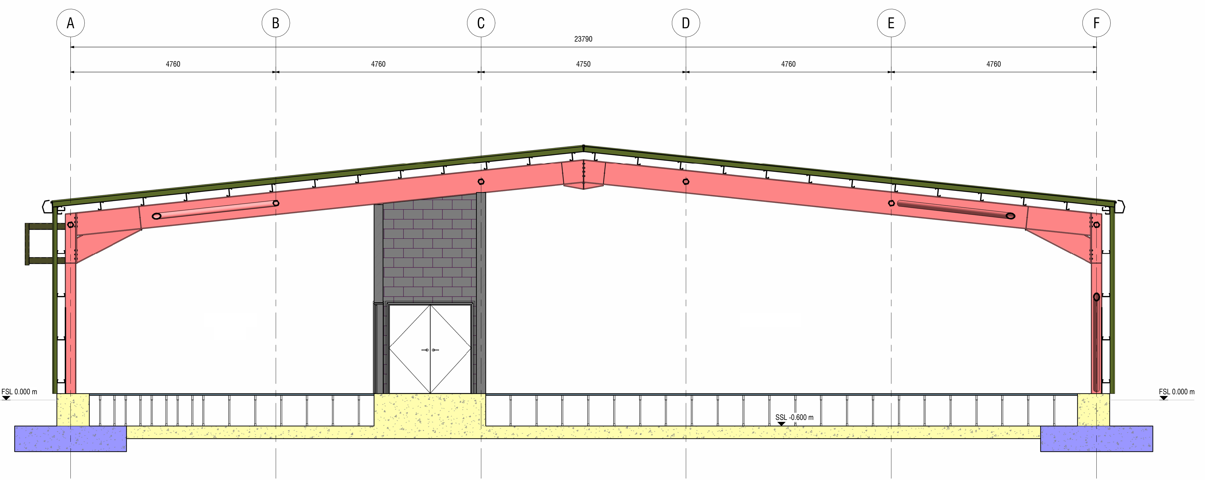
SECTION B - B (1:50)
