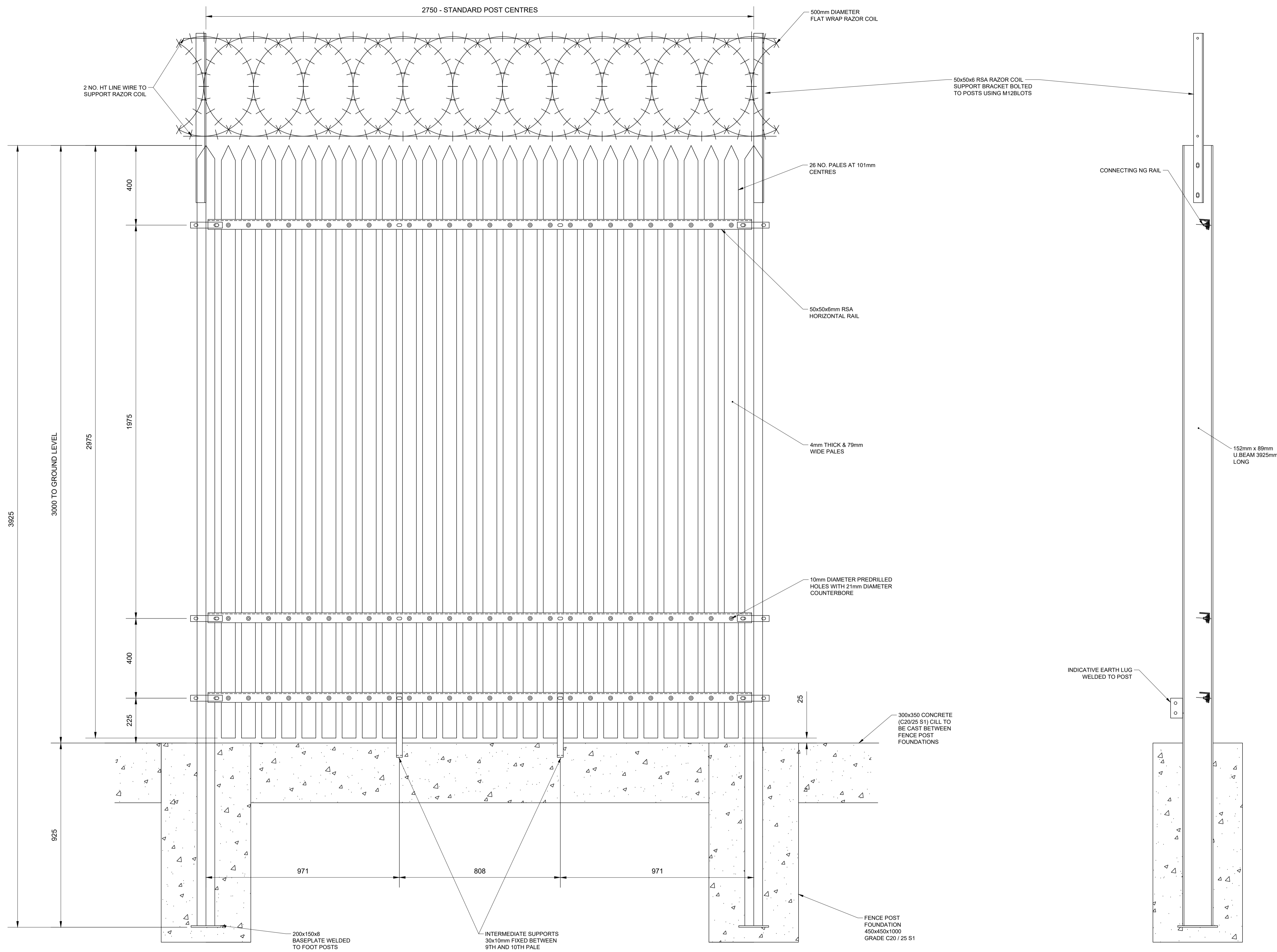
TYPICAL ELEVATION OF STANDARD FENCE PANEL SCALE 1:10
