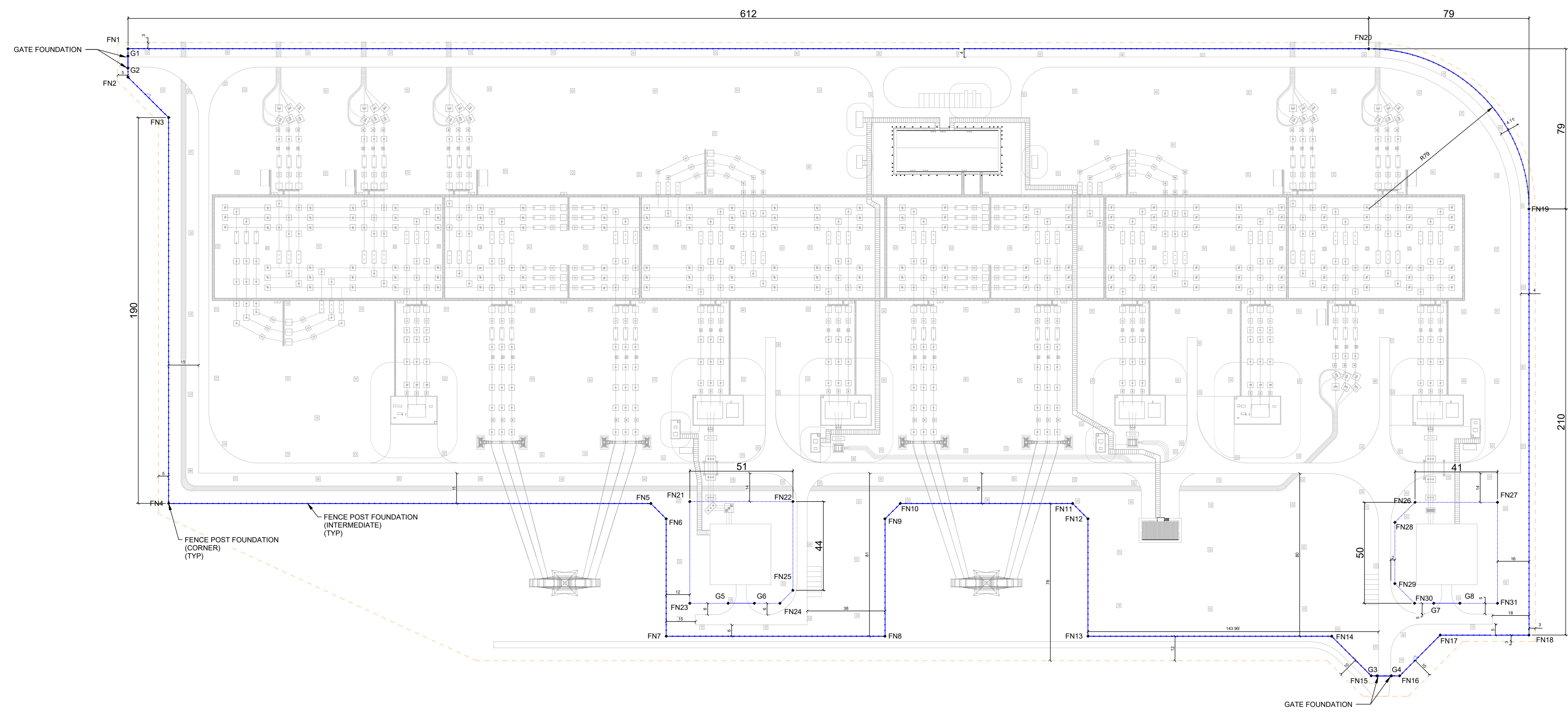
SECURITY FENCING AND GATE - LAYOUT 1:1000
