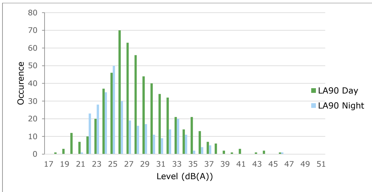
Figure 4: Measured Background LA 90 Noise Levels for BGN 4
