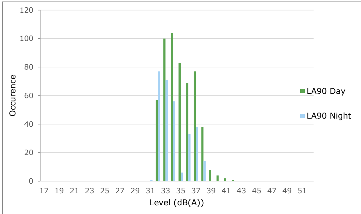
Figure 5: Measured Background LA 90 Noise Levels for BGN 5
