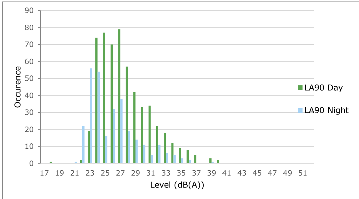
Figure 3: Measured Background LA 90 Noise Levels for BGN 3
