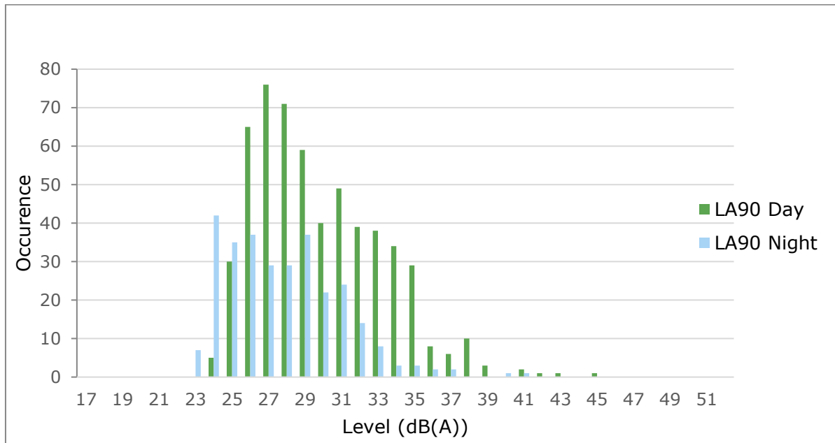
Figure 2: Measured Background LA 90 Noise Levels for BGN 2
