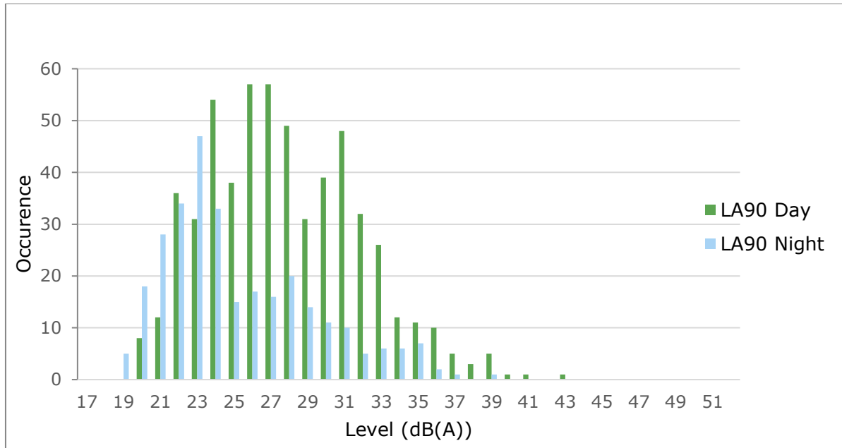
Figure 1: Measured Background LA 90 Noise Levels for BGN 1
