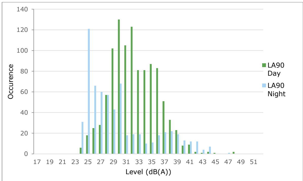
Figure 6: Measured Background LA 90 Noise Levels for BGN 6
