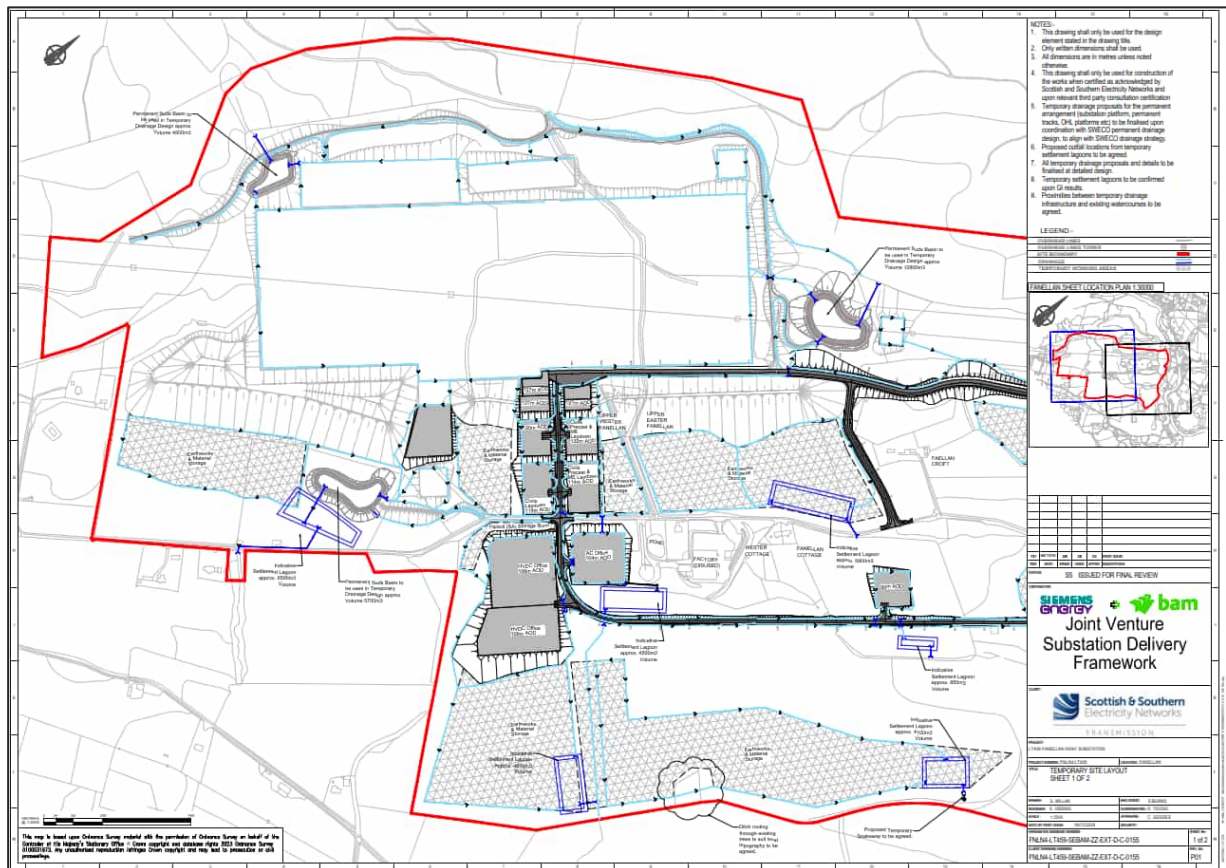
Figure 3-1 - Indicative Temporary Site Layout (Frame 1)
