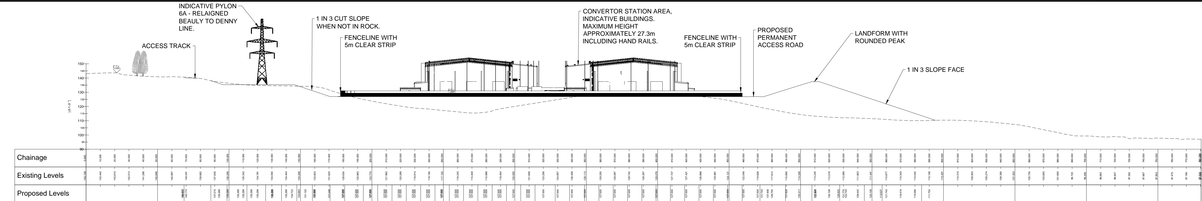
INDICATIVE SECTION A-A SCALE 1:1250
