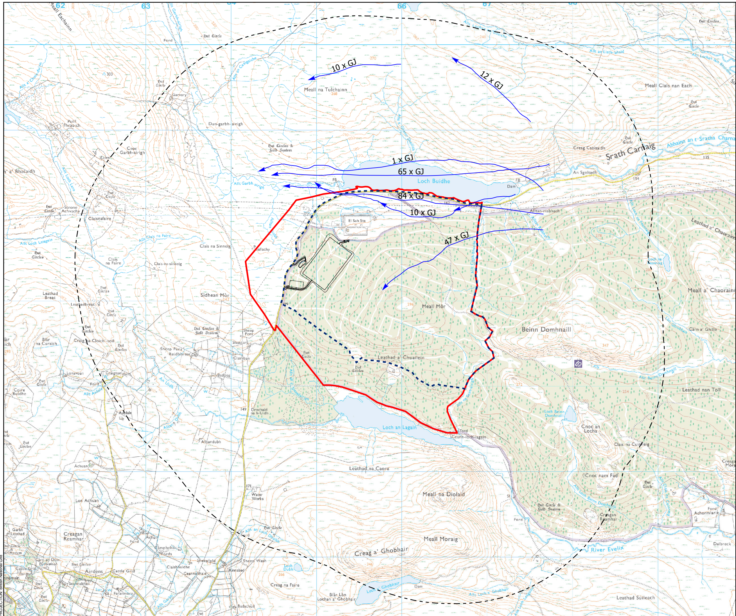
Figure 8.5 Winter Goose Flight Activity within Survey Area [2 km]
